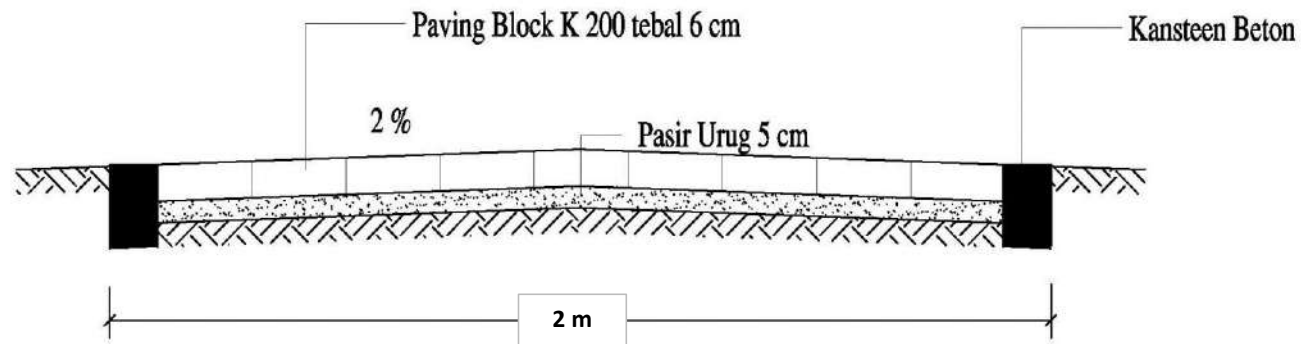
DETAIL PAVING CONBLOK
